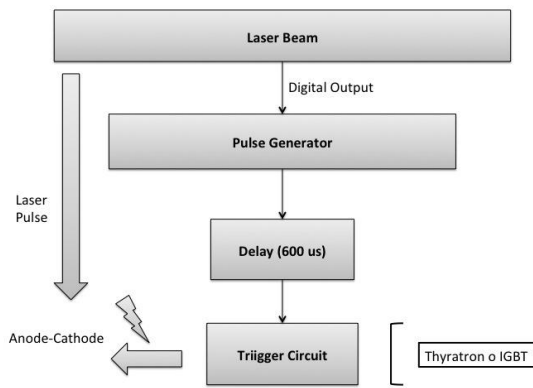
Figure 1: Synchronization Layout. Digital output is generated simultaneously with laser beam and is sent to the Pulse Generator as trigger for obtaining a new signal delayed about 600 us which controls the trigger circuit.
