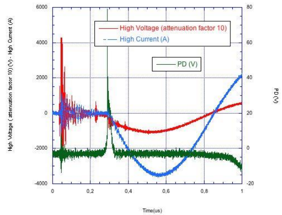
Figure 2: Experimental Signals in vacuum of 10 -3 mbar with 15kV of Power supply: In blue line, High Current Signal, in red line the High Voltage with attenuation factor of 10 and in green line, the x-ray emission.
