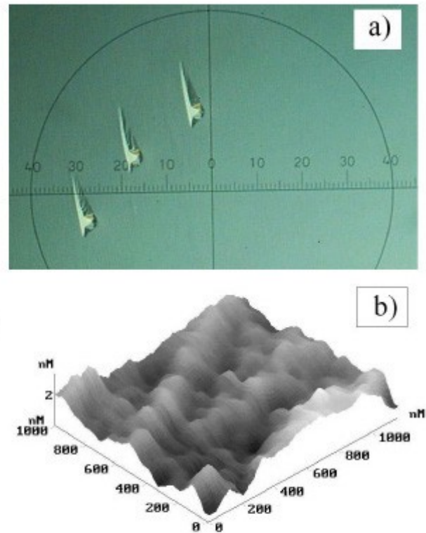
Fig. 2. Optical (a) and AFM (b) images of the CdSSe/CdS MQW structure #177. Small scale division of optical image is 2.5 μm. RMS roughness is 0.48 nm.
